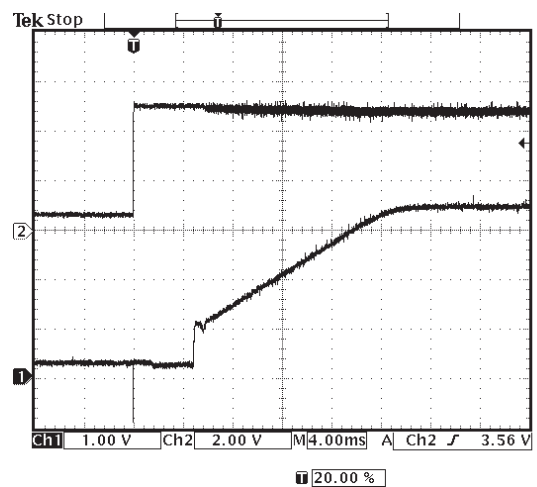
Figure 38: Typical Power-up Characteristic (Channel 1: V_o , Channel 2: V_{in} )
